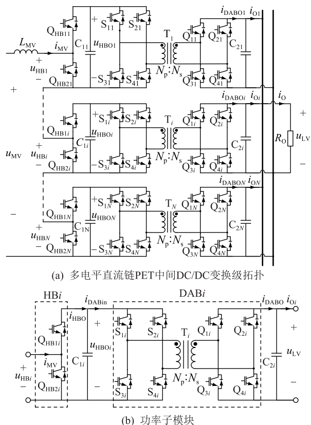
图 1 多电平直流链 PET 中间 DC/DC 变换级拓扑 Fig.1 Topology of the middle DC/DC stage for the multi-level DC-link PET
